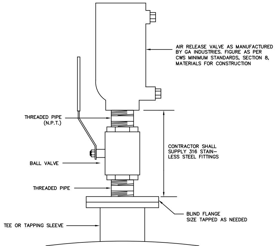
AIR RELEASE VALVE FOR WATER SYSTEM
